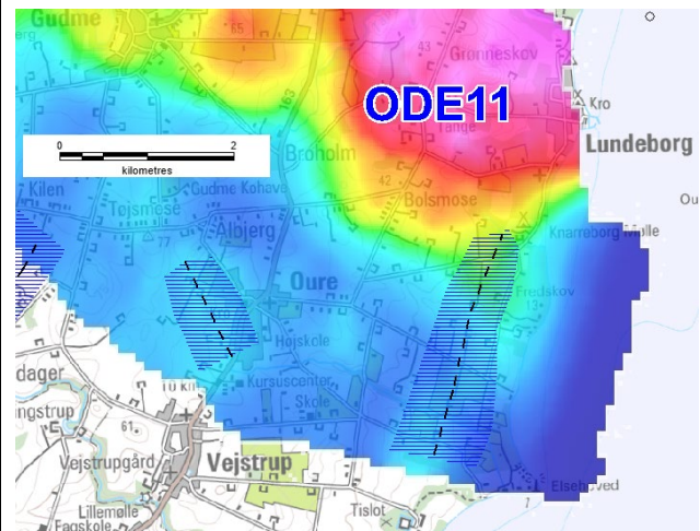
Figur 2: TEM middelmodstand kote -35 m
